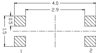
PCB.焊接图 PCB.WELDING DRAWING
